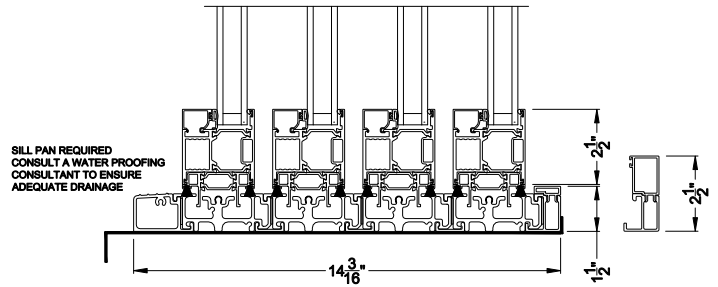
VUE COLLECTION MULTI-SLIDE PATIO DOOR (4701) Vertical Section - with Sill Riser - 4 or Bi-parting 8 Panel Door
