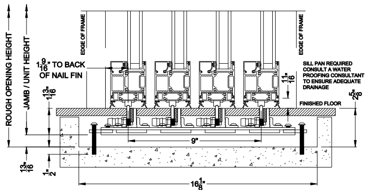
VUE COLLECTION MULTI-SLIDE PATIO DOOR (4701) Vertical Section - with Drainage T-track sill - 4 or Bi-parting 8 Panel Door
