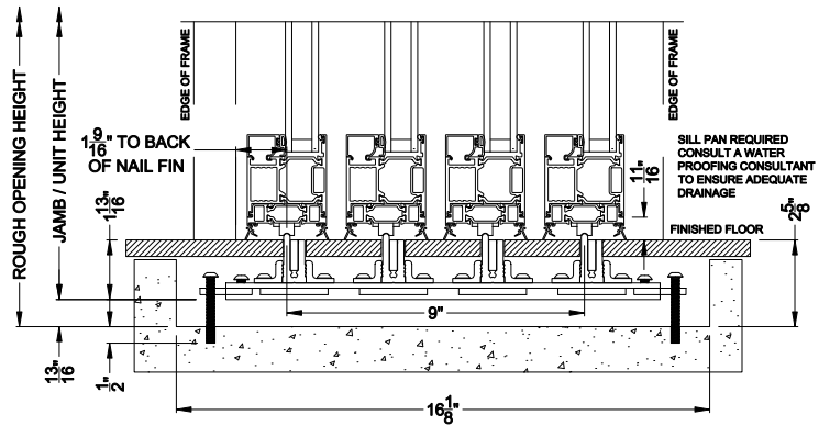
VUE COLLECTION MULTI-SLIDE PATIO DOOR (4701) Vertical Section - with T-track sill - 4 or Bi-parting 8 Panel Door
