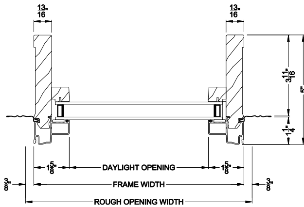
CLASSIC SERIES DIRECT-SET Horizontal Section
