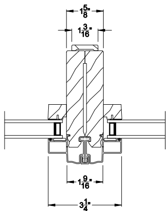
CLASSIC SERIES DIRECT-SET Vertical Mull Section
