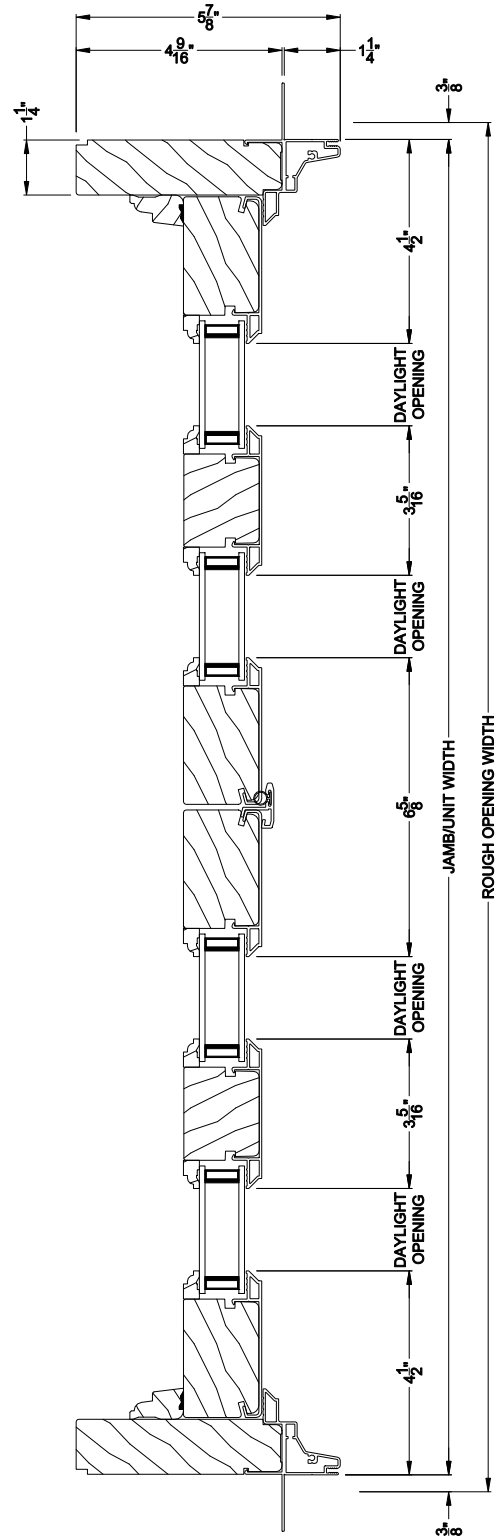
PREMIUM SLIDING DOOR TRANSOM 4 PANEL (8313) Horizontal Section
