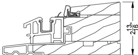
Standard Sill
