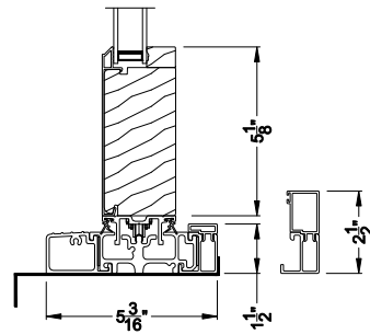
PREMIUM 2-1/4" MULTI-SLIDE PATIO DOOR (8725) Vertical Section - with Sill Riser - 1 or Bi-parting 2 Panel Door
