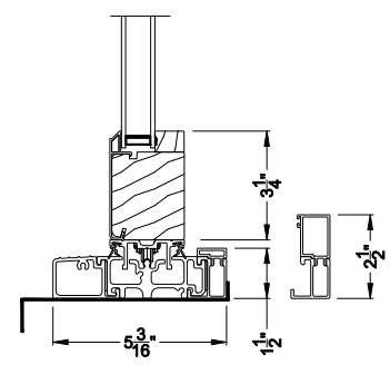
CONTEMPORARY 2-1/4" MULTI-SLIDE PATIO DOOR (8726) Vertical Section - with Sill Riser - 1 or Bi-parting 2 Panel Door
