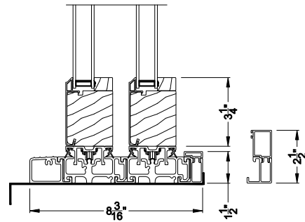
CONTEMPORARY 2-1/4" MULTI-SLIDE PATIO DOOR (8726) Vertical Section - with Sill Riser - 2 or Bi-parting 4 Panel Door
