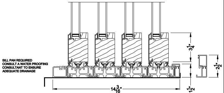
CONTEMPORARY 2-1/4" MULTI-SLIDE PATIO DOOR (8726) Vertical Section - with Sill Riser - 4 or Bi-parting 8 Panel Door
