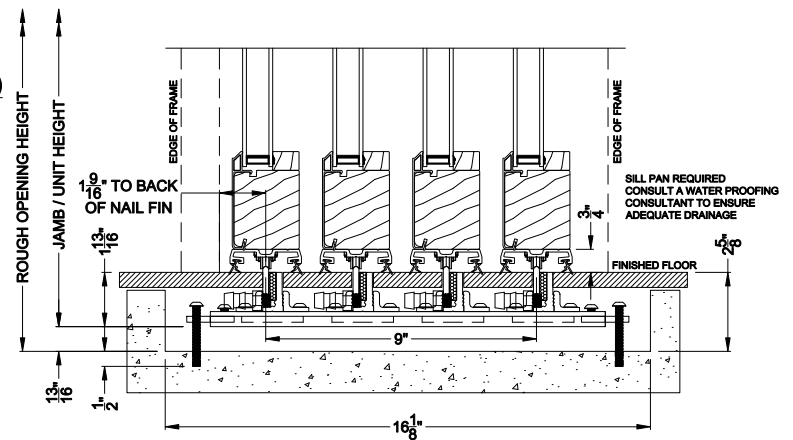
CONTEMPORARY 2-1/4" MULTI-SLIDE PATIO DOOR (8726) Vertical Section - with Drainage T-track sill - 4 or Bi-parting 8 Panel Door
