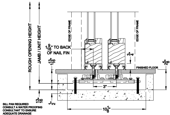
CONTEMPORARY 2-1/4" MULTI-SLIDE WINDOW (8726) Vertical Section - with Drainage T-track sill - 2 or Bi-parting 4 Panel Door
