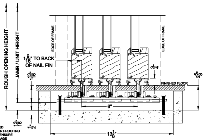
CONTEMPORARY 2-1/4" MULTI-SLIDE WINDOW (8726) Vertical Section - with Drainage T-track sill - 3 or Bi-parting 6 Panel Door
