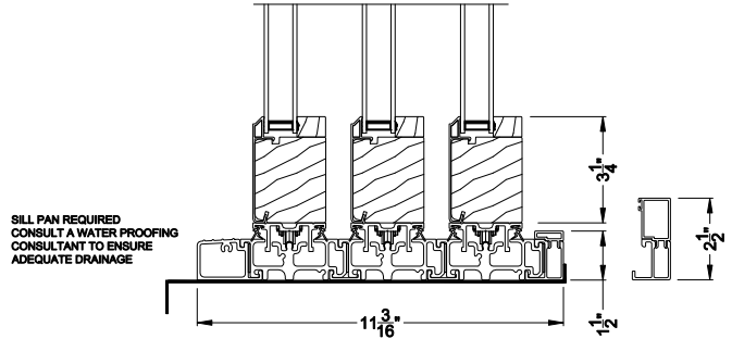
CONTEMPORARY 2-1/4" MULTI-SLIDE WINDOW (8726) Vertical Section - with Sill Riser - 3 or Bi-parting 6 Panel Door
