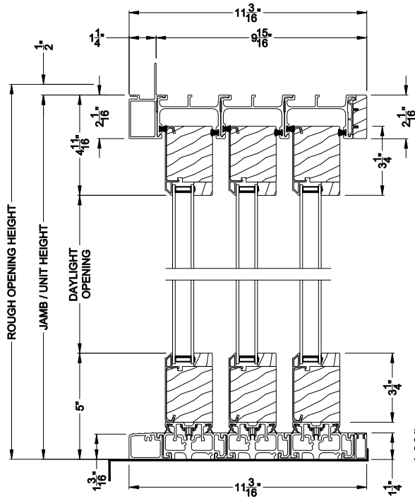
CONTEMPORARY 2-1/4" MULTI-SLIDE WINDOW (8726) Vertical Section - Standard Sill - 3 or Bi-parting 6 Panel Door
