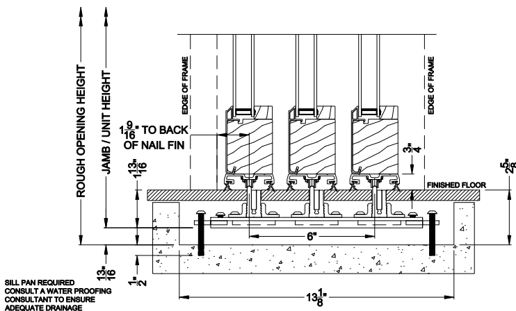
CONTEMPORARY 2-1/4" MULTI-SLIDE WINDOW (8726) Vertical Section - with T-track sill - 3 or Bi-parting 6 Panel Door
