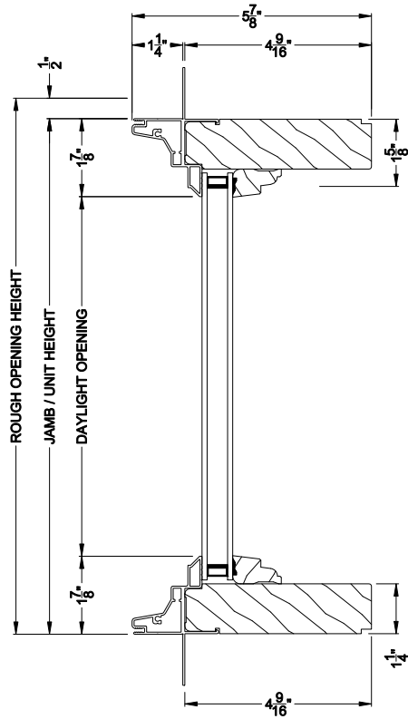
SIGNATURE SLIDING DOOR TRANSOM (8306) Vertical Section
