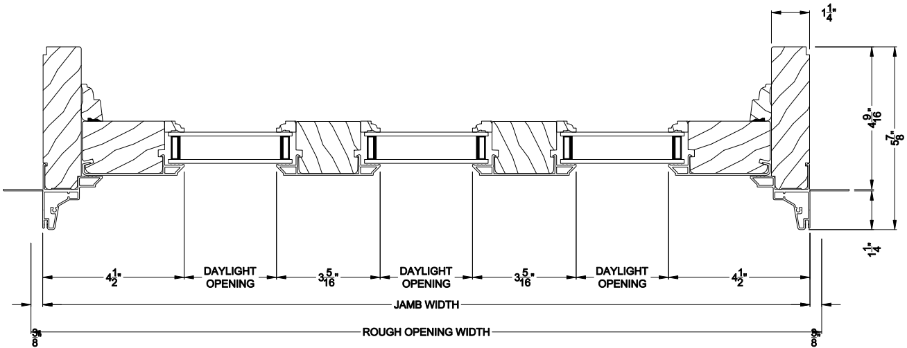
SIGNATURE SLIDING DOOR TRANSOM 3 PANEL (8313) Horizontal Section - Picture units
