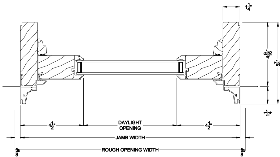
SIGNATURE SLIDING DOOR TRANSOM 1 PANEL (8313) Horizontal Section
