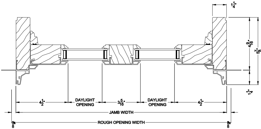
SIGNATURE SLIDING DOOR TRANSOM 2 PANEL (8313) Horizontal Section
