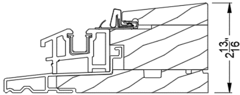
Standard Sill
