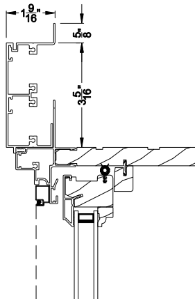
3 5/16" FLAT CASING Head Section Detail
