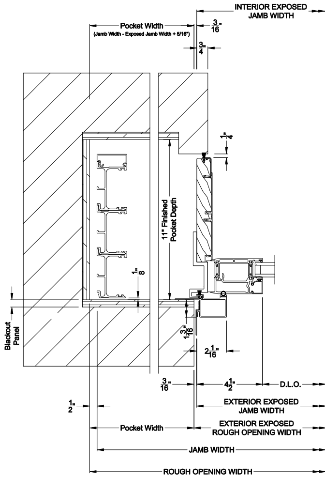
VUE COLLECTION MULTI-SLIDE WINDOW (4701) Horizontal Pocket Section - 3 or Bi-parting 6 Panel Window
