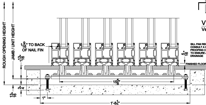
VUE COLLECTION MULTI-SLIDE WINDOW (4701) Vertical Section - with T-track sill - 6 Panel Window
