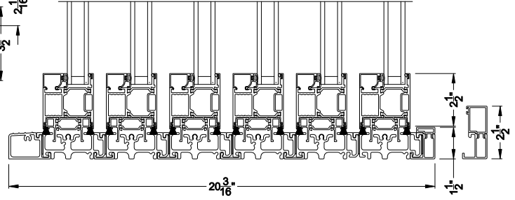
VUE COLLECTION MULTI-SLIDE WINDOW (4701) Vertical Section - with Sill Riser - 6 Panel Single Direction Window
