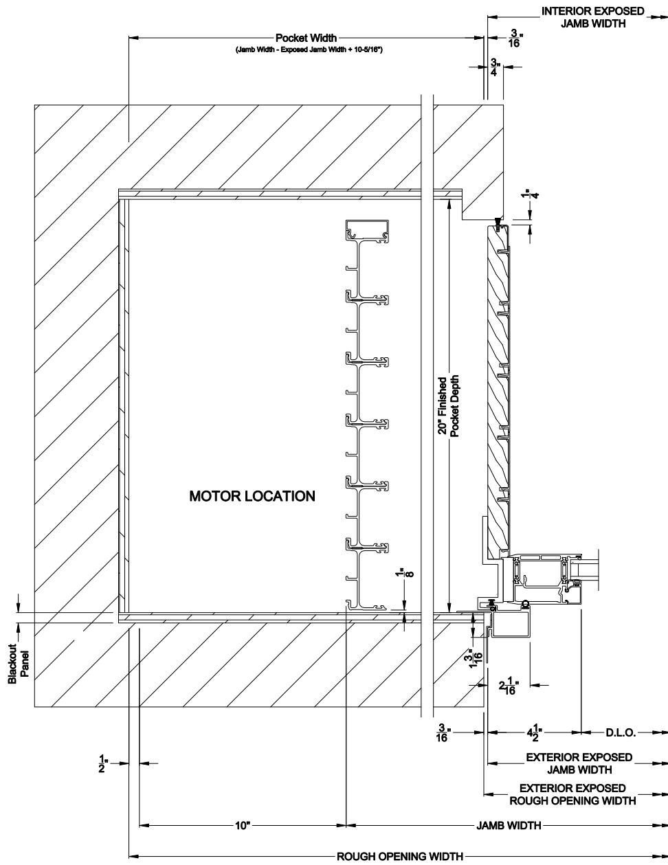
VUE COLLECTION MULTI-SLIDE WINDOW (4701) Horizontal Pocket Section - 6 Panel Single Direction Window
