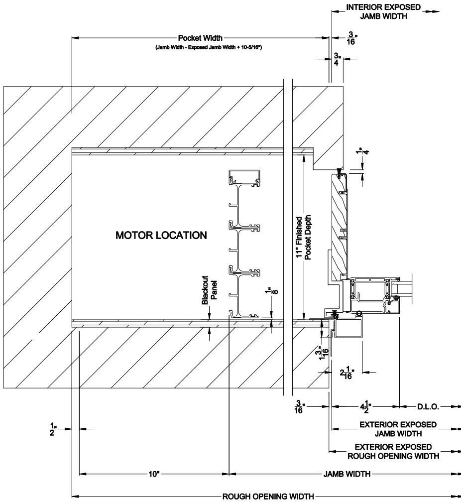
VUE COLLECTION MULTI-SLIDE WINDOW (4701) Horizontal Motorized Pocket Section - 3 or Bi-parting 6 Panel Window
