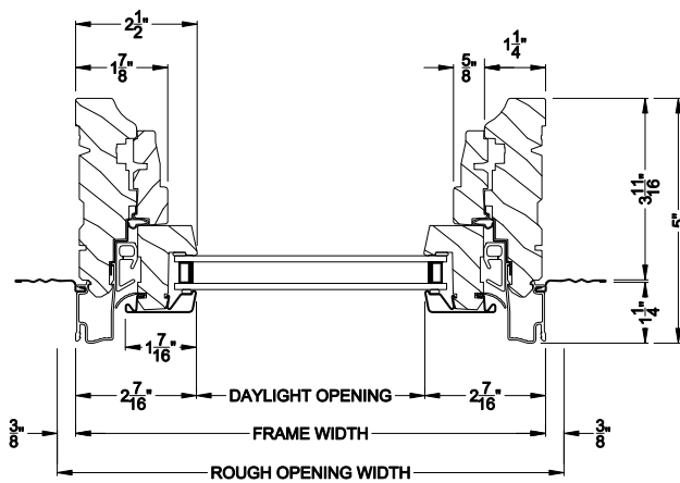
CLASSIC SERIES CASEMENT PICTURE Horizontal Section
