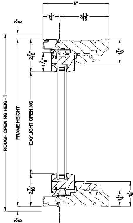
CLASSIC SERIES CASEMENT PICTURE Vertical Section
