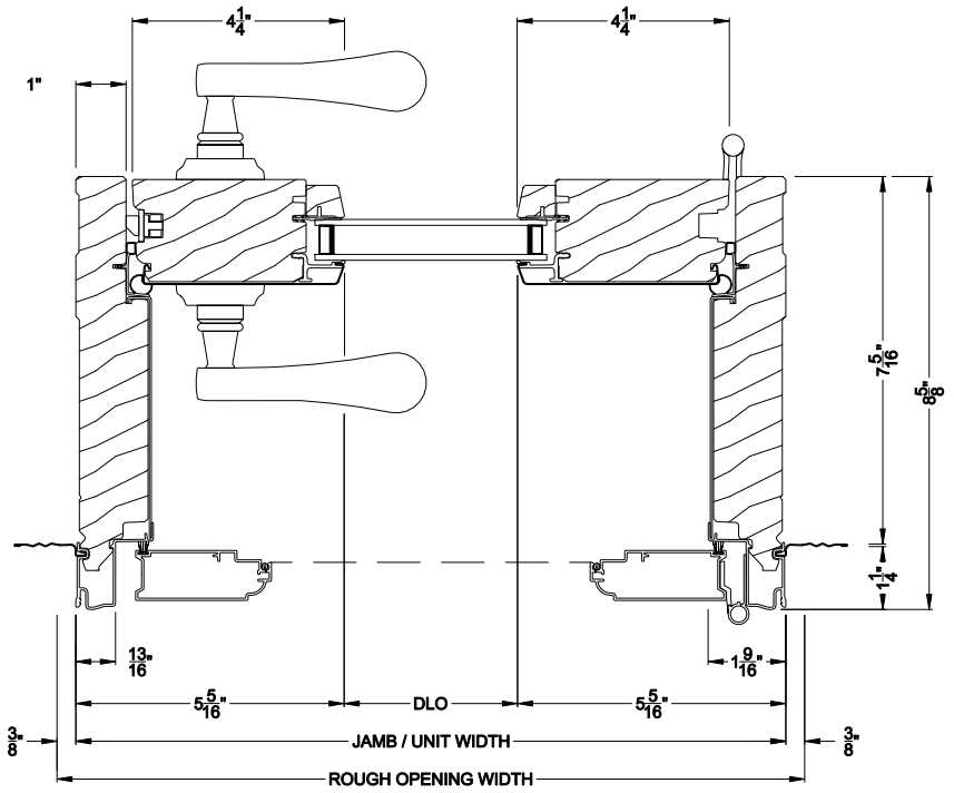
CLASSIC INSWING DOOR Horizontal Section - Single Door - 7-5/16" jamb (max) Shown with Optional Hinged Screen
