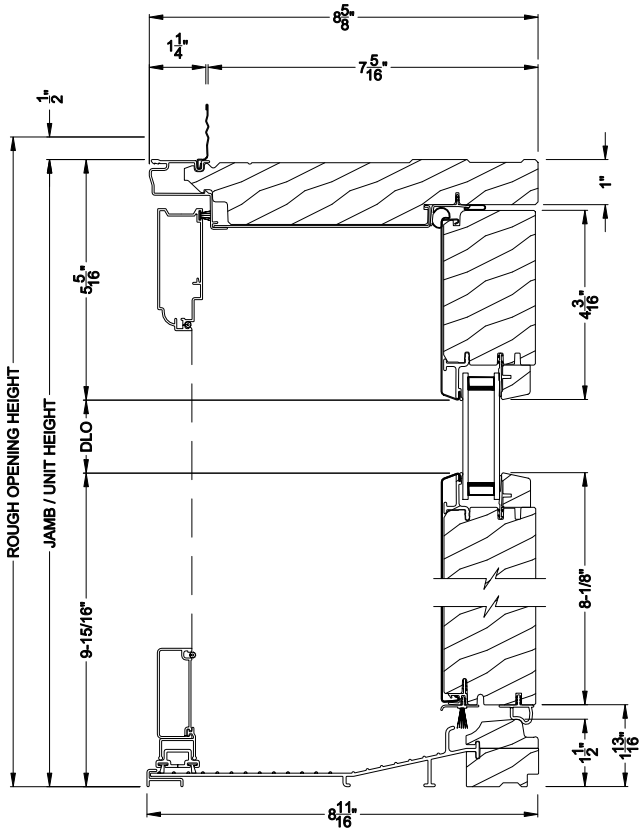
CLASSIC INSWING DOOR Vertical Section - 7-5/16" jamb (max) Shown with Optional Hinged Screen
