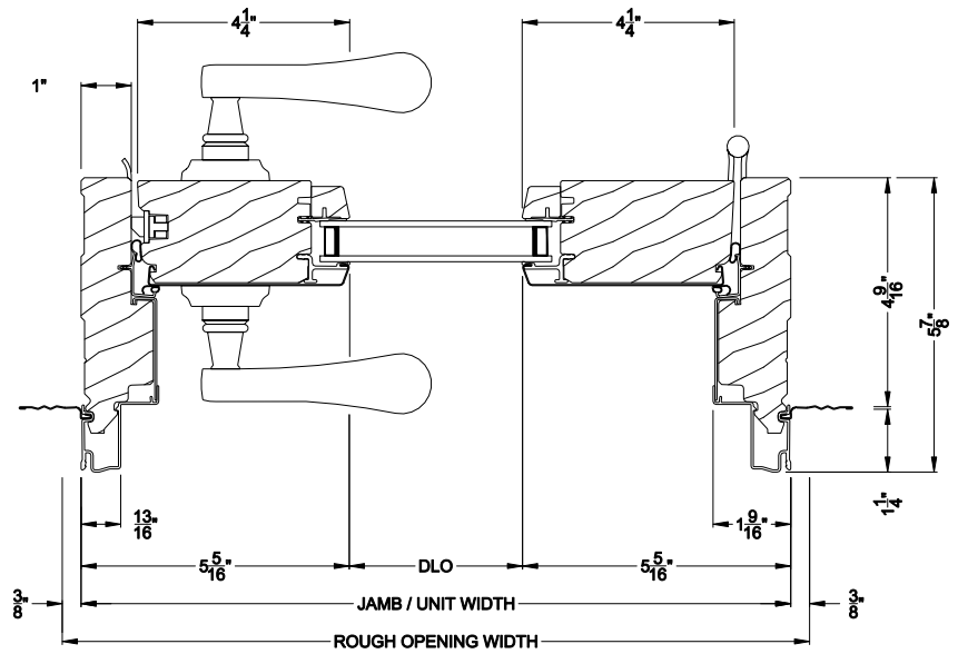
CLASSIC SERIES INSWING DOOR Horizontal Section - Single Door
