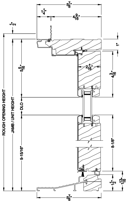
CLASSIC SERIES INSWING DOOR Vertical Section
